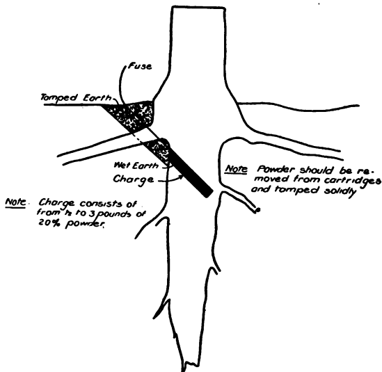
Fig. 23. Diagram Showing a Section of a Tap-Rooted Stump and a Charge in Position for Blasting
